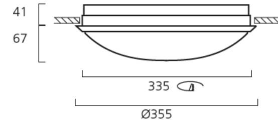
Giotto 335 Recessed
